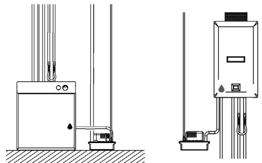
Hydraulic connections
