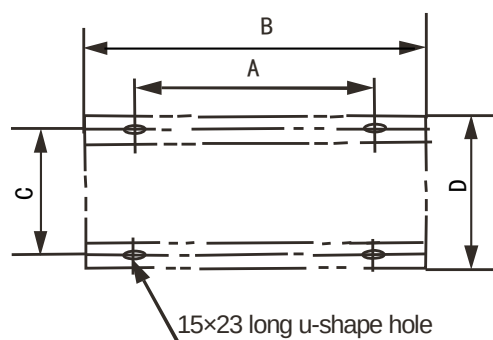
Figure 3-2.7: Expansion bolt positioning
