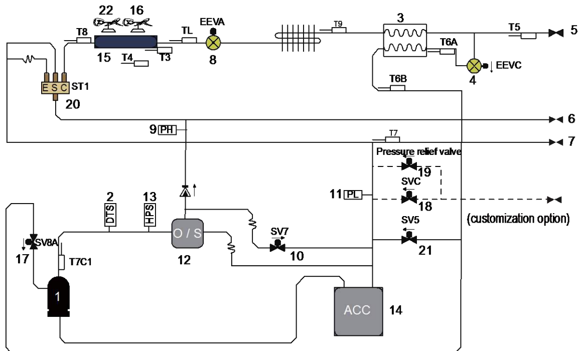
Figure 2-5.2: 14HP/16HP/18HP piping diagram
