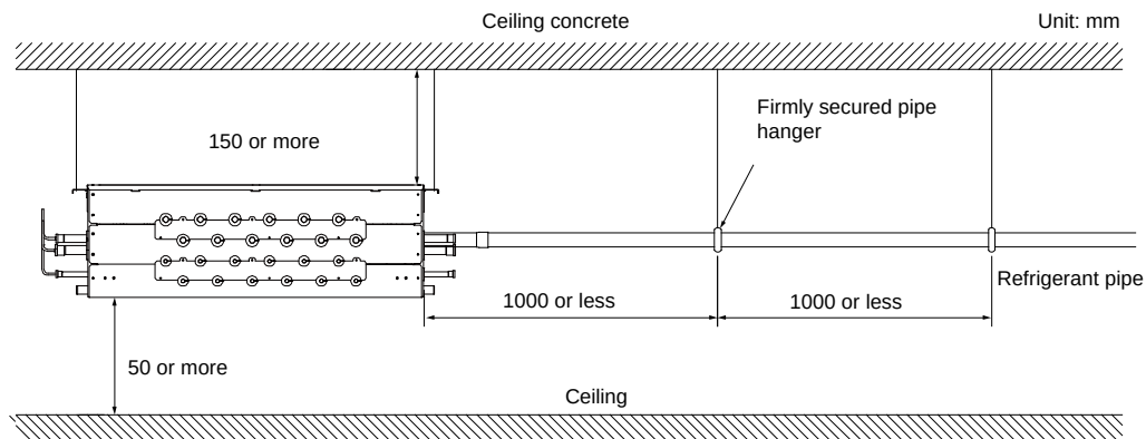
Figure 3-2.9: MS04-12 installation requirement (unit: mm)
