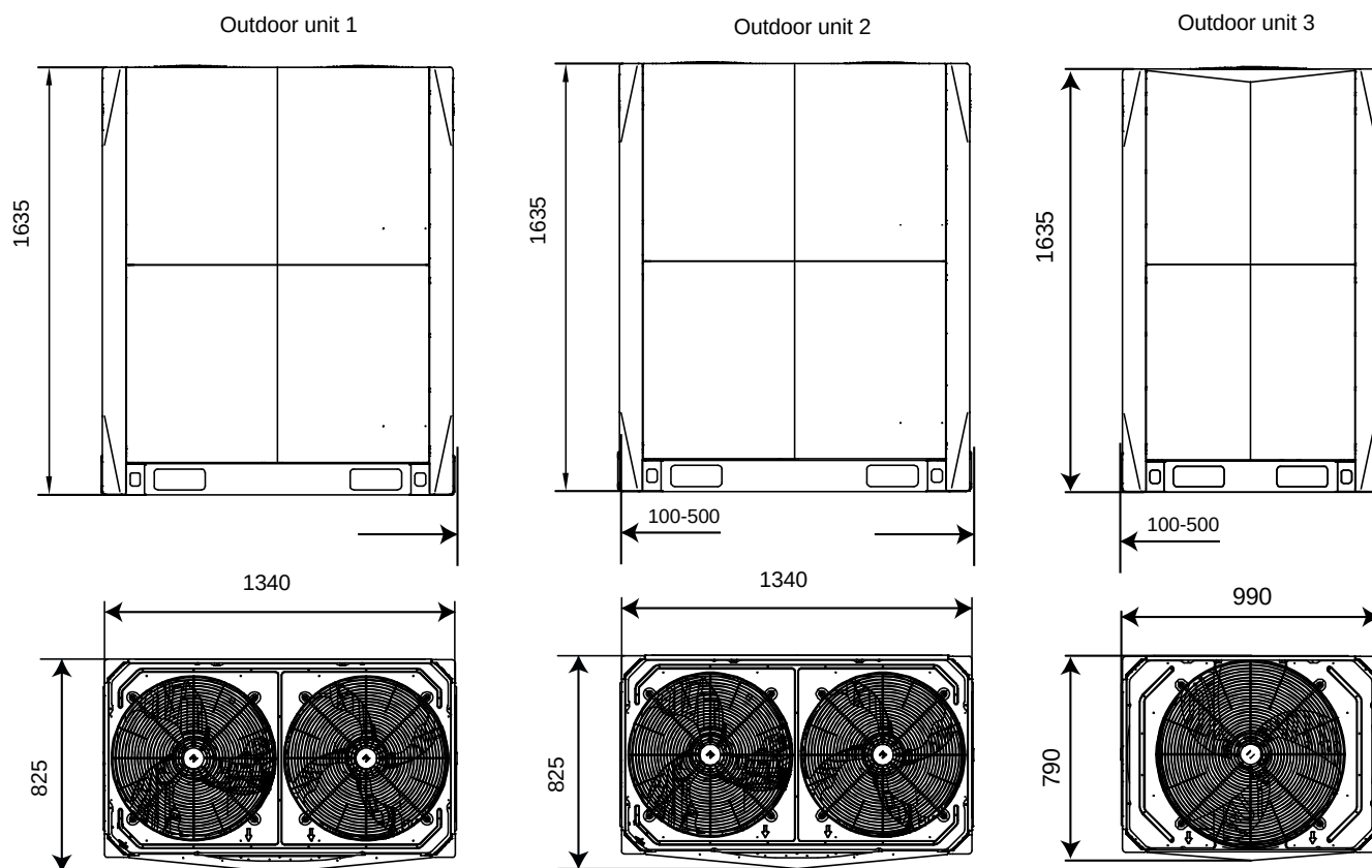
Figure 2-2.8: 46/48/50/52/54HP dimensions (unit: mm)
