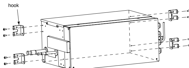
Figure 3-2.16: Step 2 for wall-mounted type replacing
