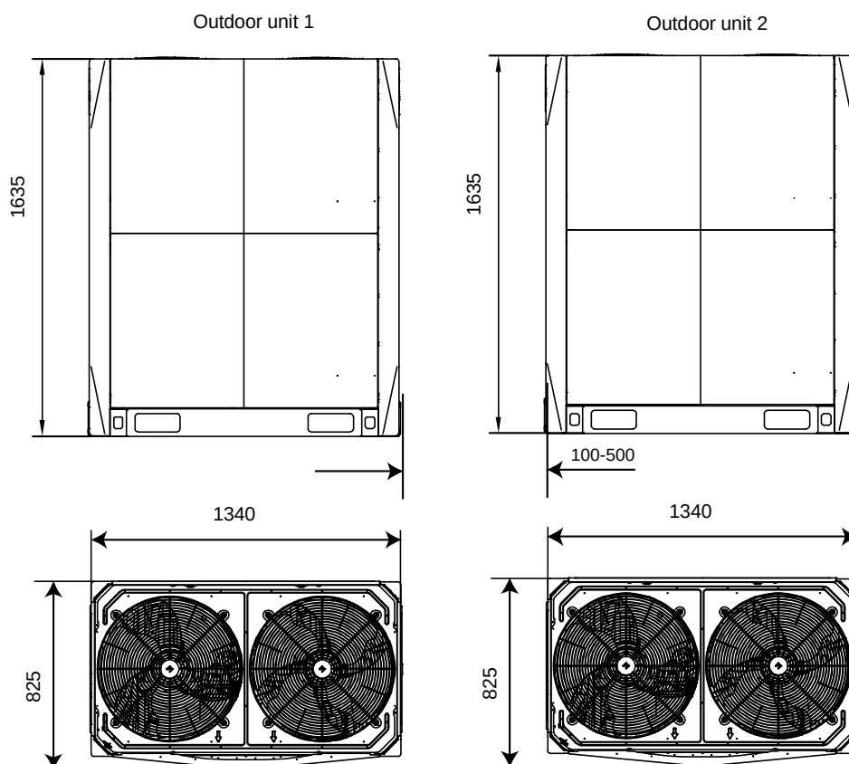
Figure 2-2.6: 38/40HP dimensions (unit: mm)
