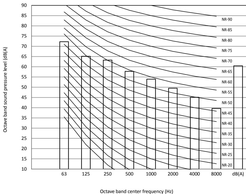
Figure 2-11.4: 12HP octave band level
