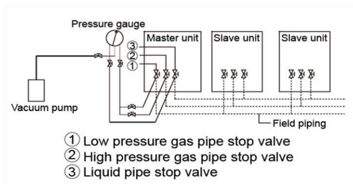
Figure 3-5.14: Vacuum drying
