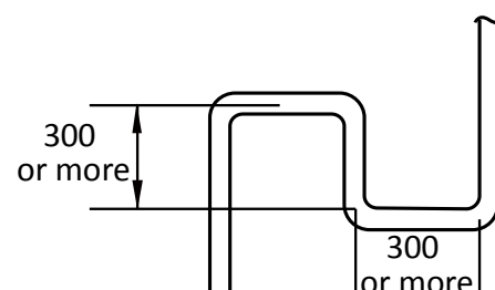
Figure 3-4.1: Oil return bend (unit: mm)
