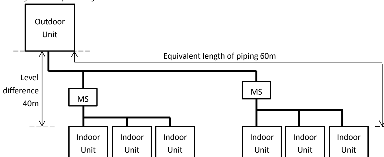
Figure 1-6.2: System diagram
