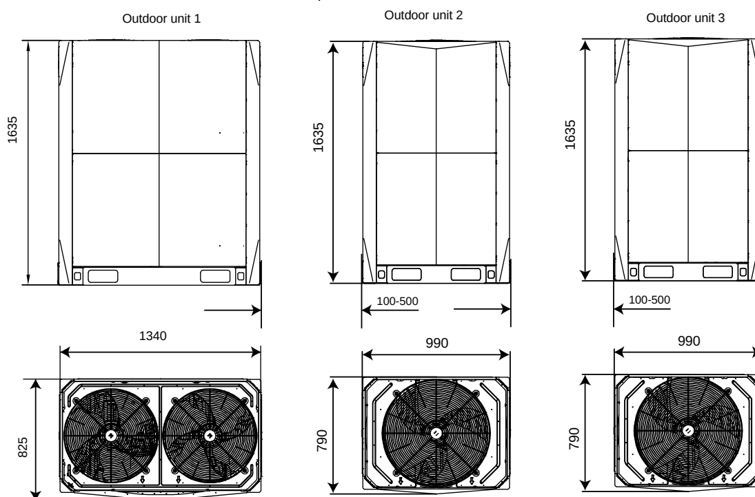
Figure 2-2.6: 38/40HP dimensions (unit: mm)
