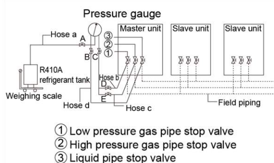
Figure 3-8.1: Charging refrigerant
