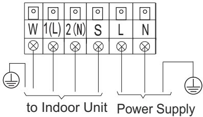
Outdoor unit terminals
