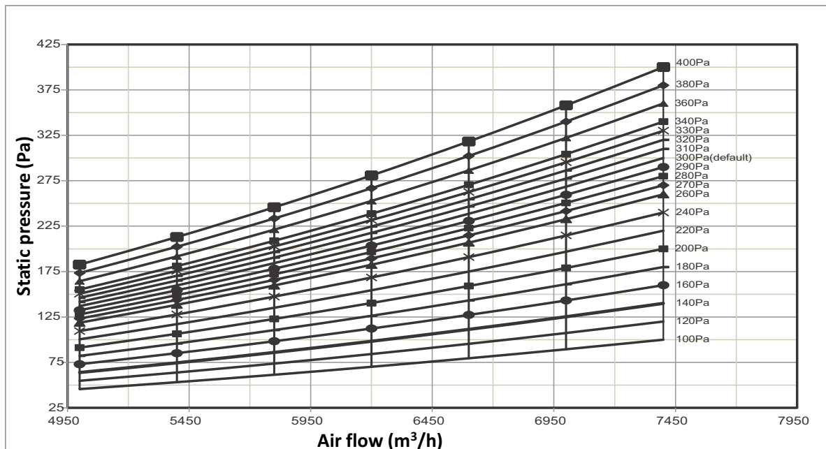
Figure 6.4: Model 560
