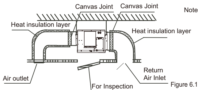
Figure 6.1: Model 160
