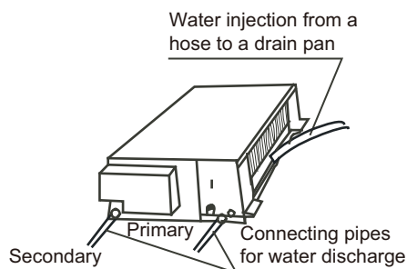
Figure 5.4 Verify water discharge
