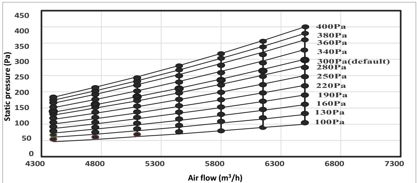
Figure 6.3: Models 400 / 450
