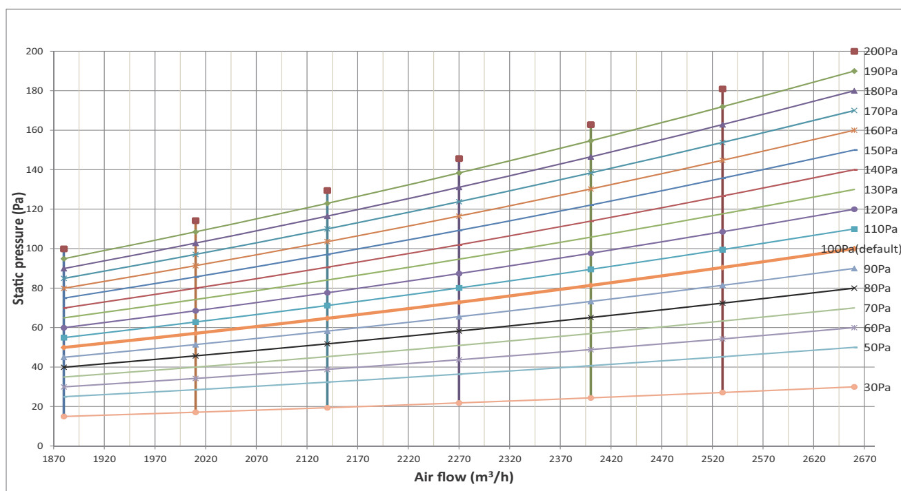
Figure 6.2: Models 200 / 250 / 280
