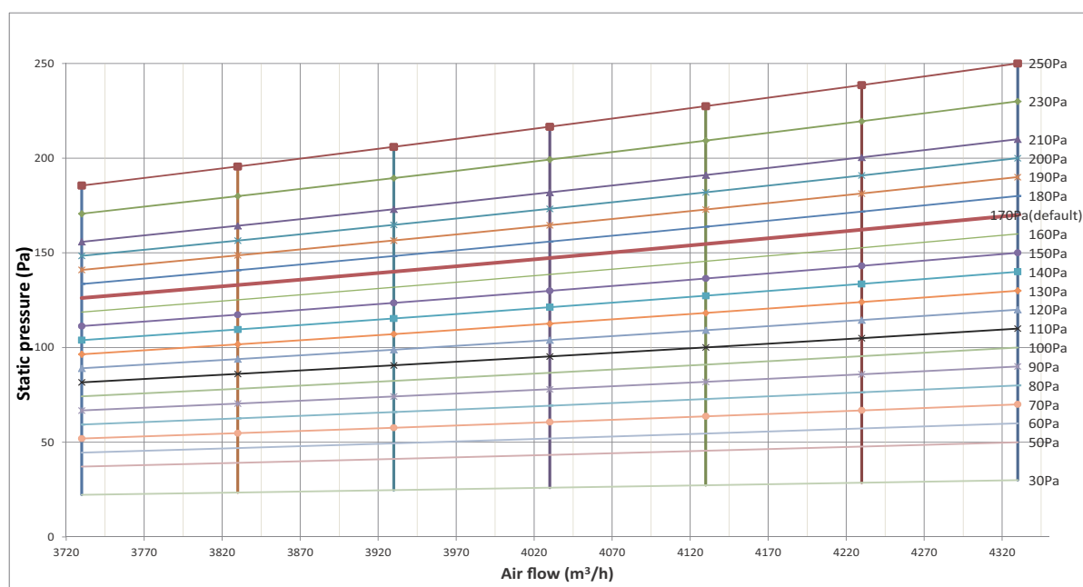
Figure 6.2: Models 200 / 250 / 280
