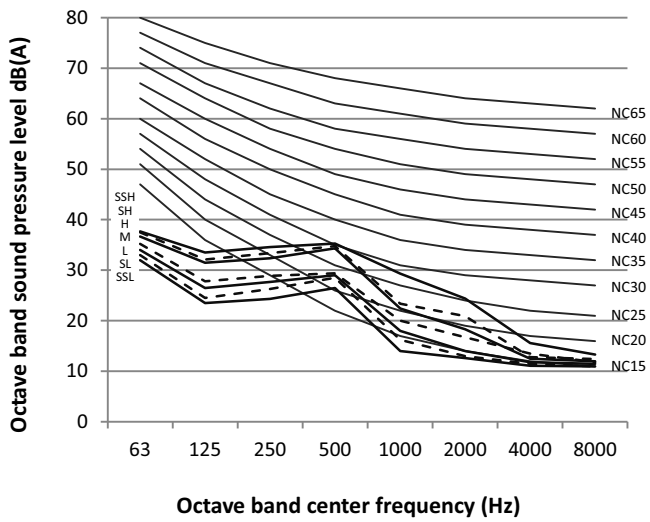
Figure 8.4: MVD-80(90)DLDN1 octave band levels
