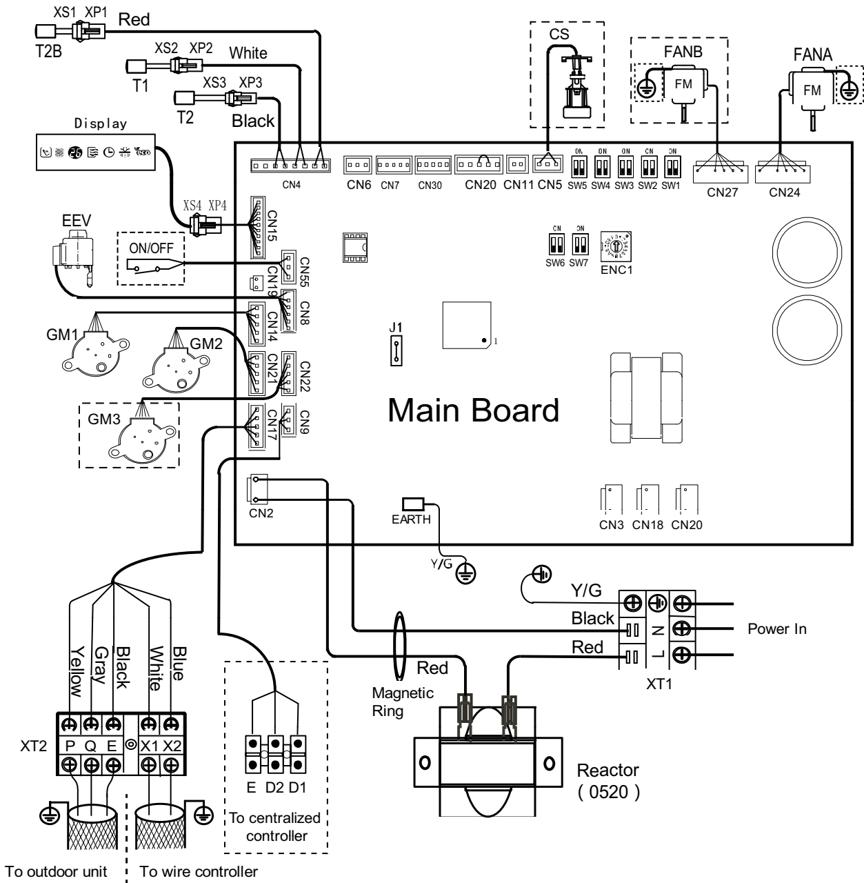
Figure 5.1: Ceiling & floor wiring diagram
