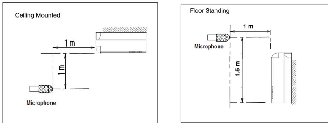
Figure 8.1: Ceiling & floor sound pressure level measurement
