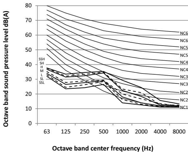
Figure 8.2: MVD-36DLDN1 octave band levels
