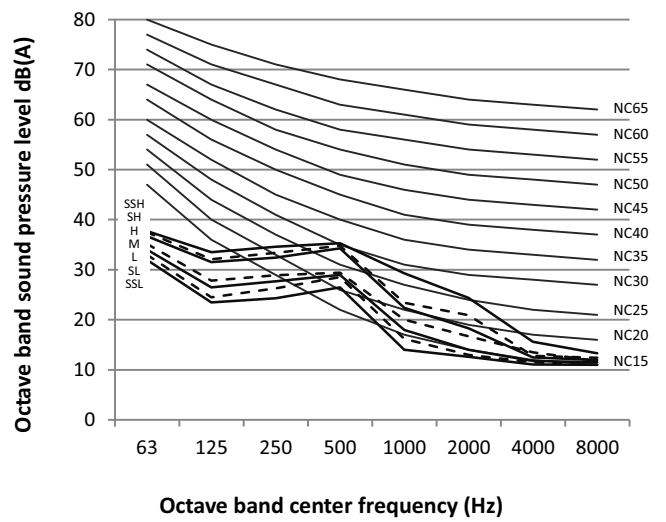
Figure 8.5: MVD-112(140)DLDN1 octave band levels
