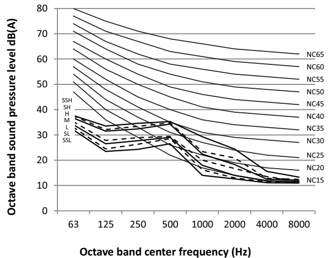
Figure 8.3: MVD-45(56,71)DLDN1 octave band levels
