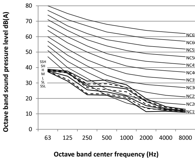
Figure 8.2: MVD-22(28)GDN1 octave band levels
