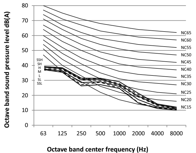
Figure 8.3: MVD-36GDN1 octave band levels
