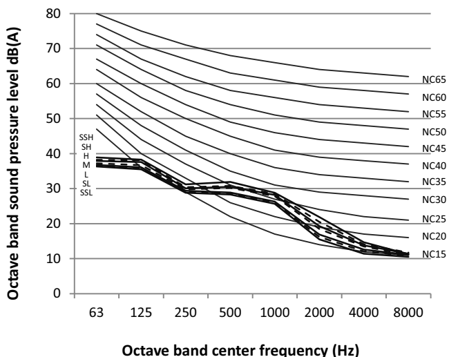
Figure 8.6: MVD-71(80)GDN1 octave band levels
