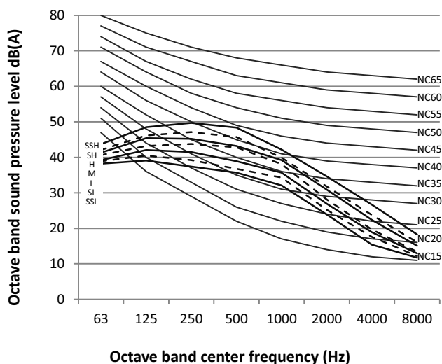
Figure 8.7: MVD-90GDN1 octave band levels
