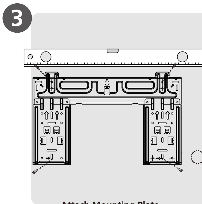
Attach Mounting Plate
