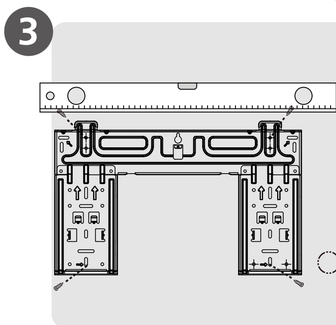
Attach Mounting Plate
