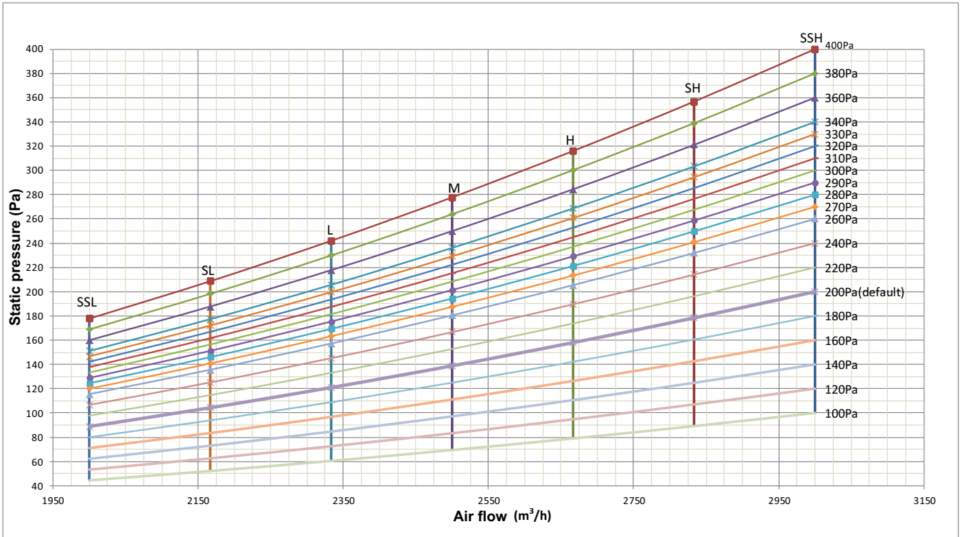
Figure 6.2: Models 200 / 250 / 280
