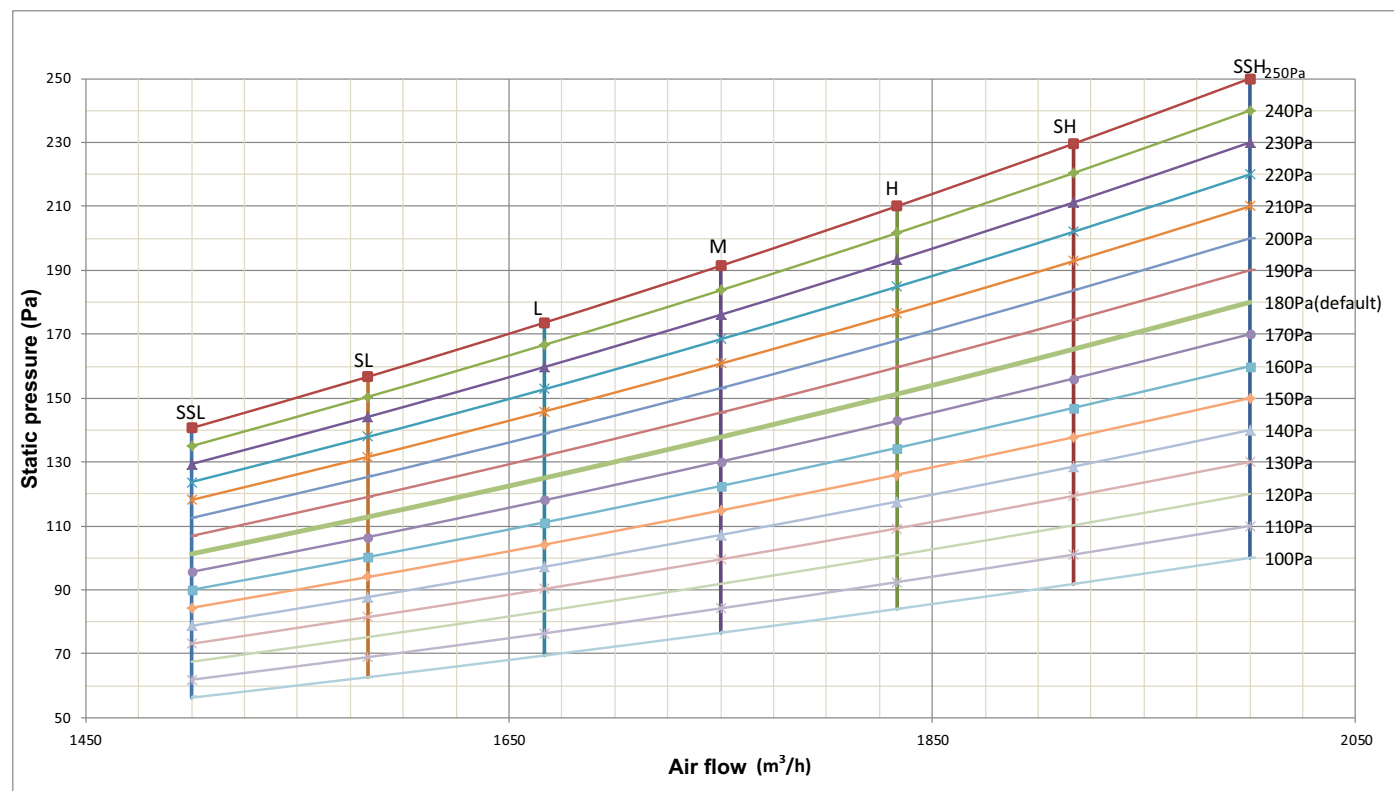
Figure 6.1: Models 125 / 140
