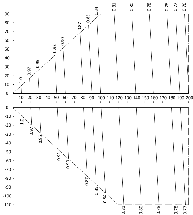
Figure 2-8.29: MVD-V5X1790(1845)W/V2GN1 rate of change in cooling capacity
