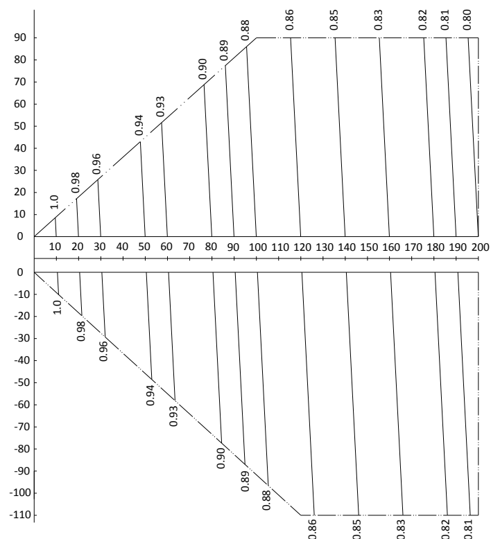
Figure 2-8.19: MVD-V5X1285W/V2GN1 rate of change in cooling capacity
