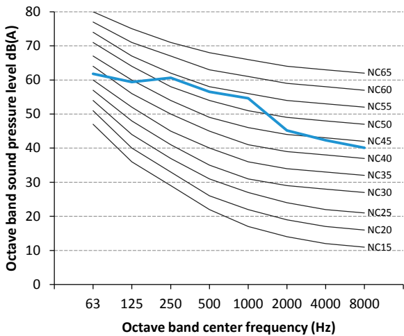
Figure 2-10.3 MVD-V5X280W/V2GN1 octave band level
