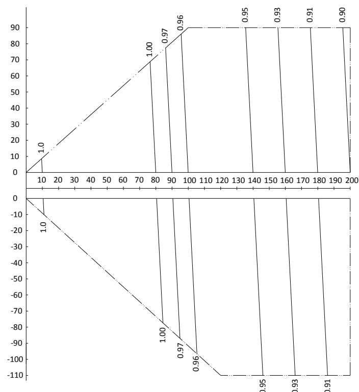
Figure 2-8.32: MVD-V5X1900W/V2GN1 rate of change in heating capacity
