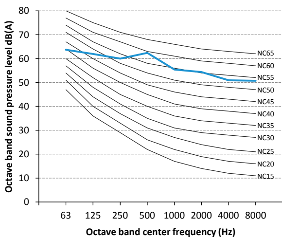
Figure 2-10.8 MVD-V5X560W/V2GN1 octave band level
