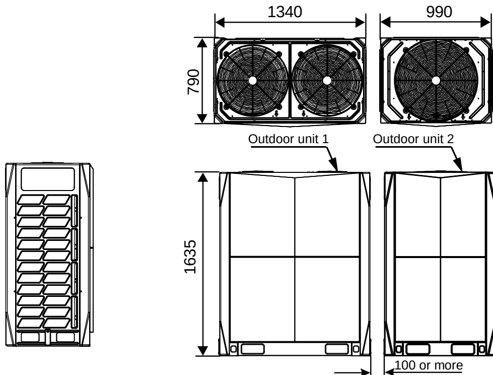
Figure 2-2.4: MVD-V5X730(780, 840, 895, 950)W/V2GN1 dimensions (unit: mm)
