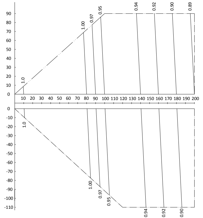
Figure 2-8.18: MVD-V5X1175(1230)W/V2GN1 rate of change in heating capacity
