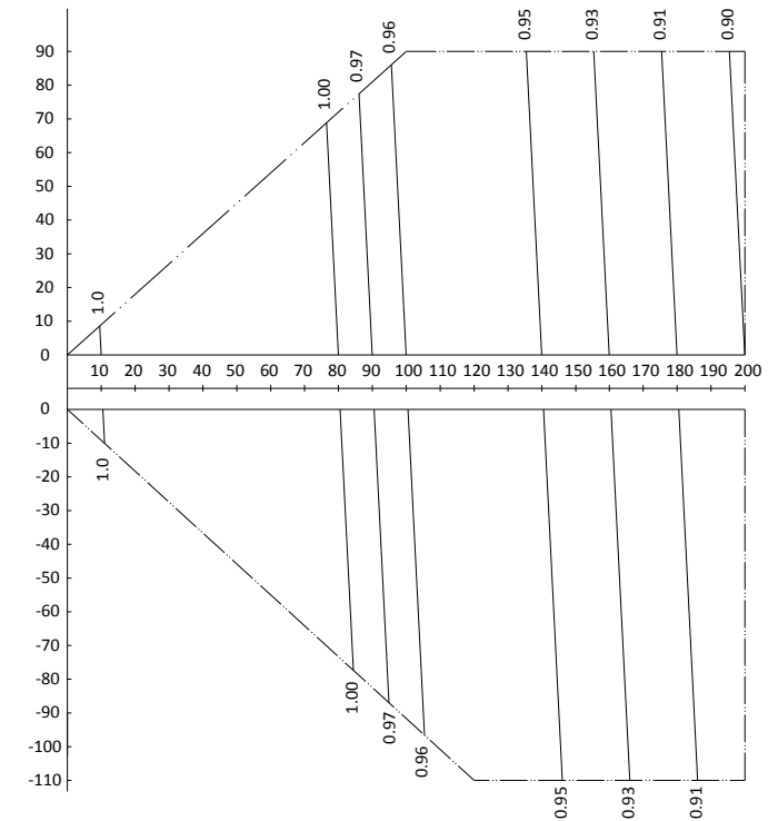
Figure 2-8.26: MVD-V5X1615W/V2GN1 rate of change in heating capacity
