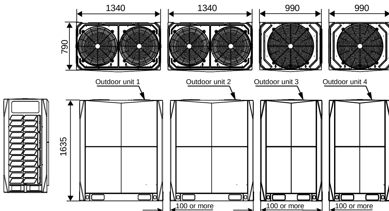
Figure 2-2.9: MVD-V5X1900W/V2GN1 dimensions (unit: mm)
