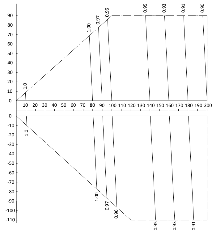
Figure 2-8.4: MVD-V5X400(450, 500)W/V2GN1 rate of change in heating capacity
