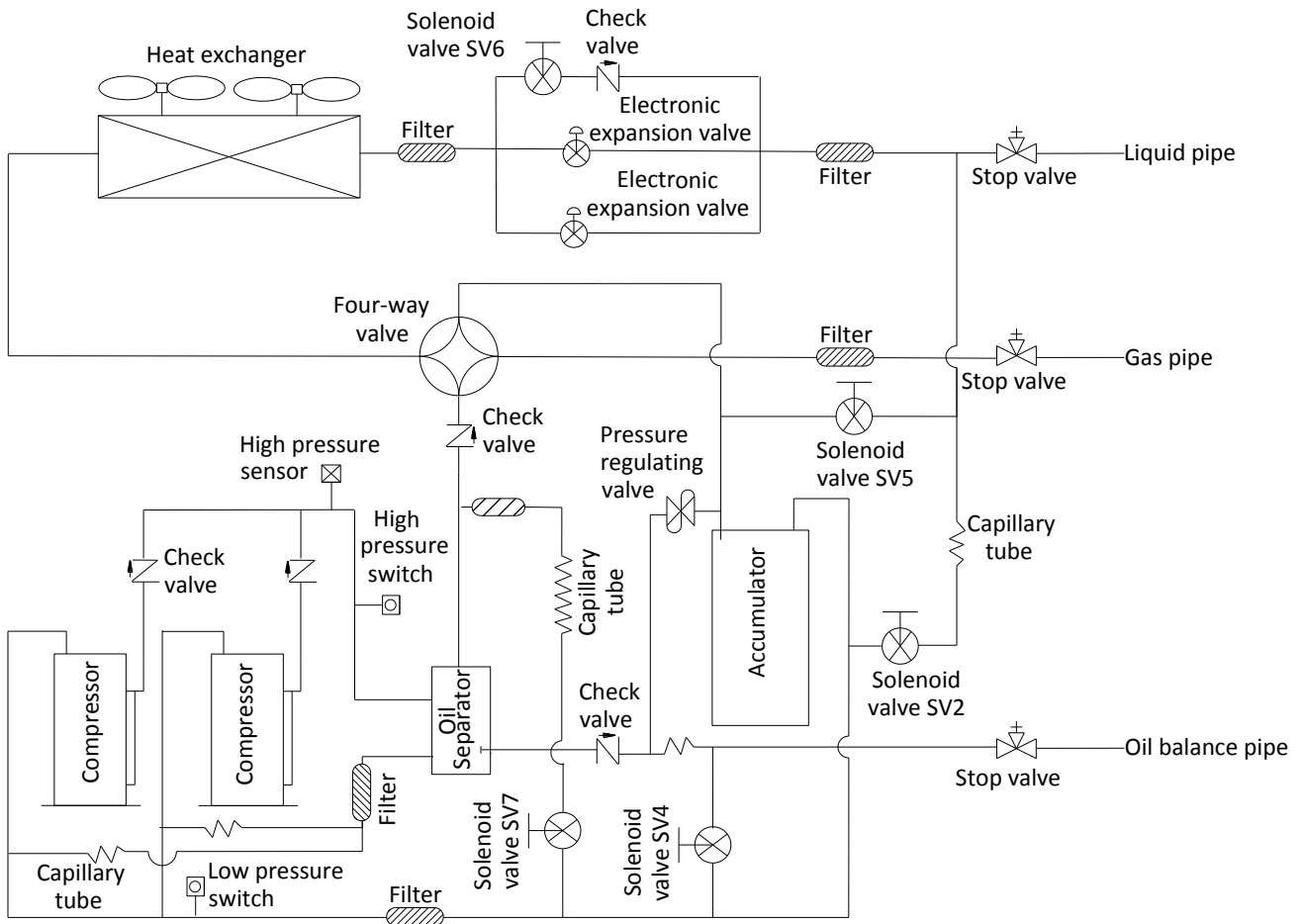
Figure 2-4.3: MVD-V5X500(560, 615)W/V2GN1 piping diagram
