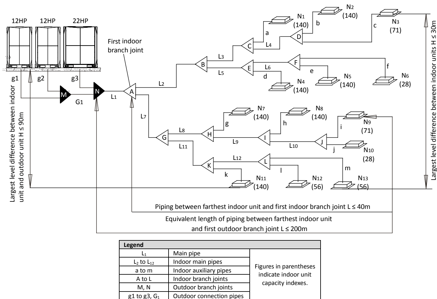
Figure 3-4.2: Permitted refrigerant piping lengths and level differences
