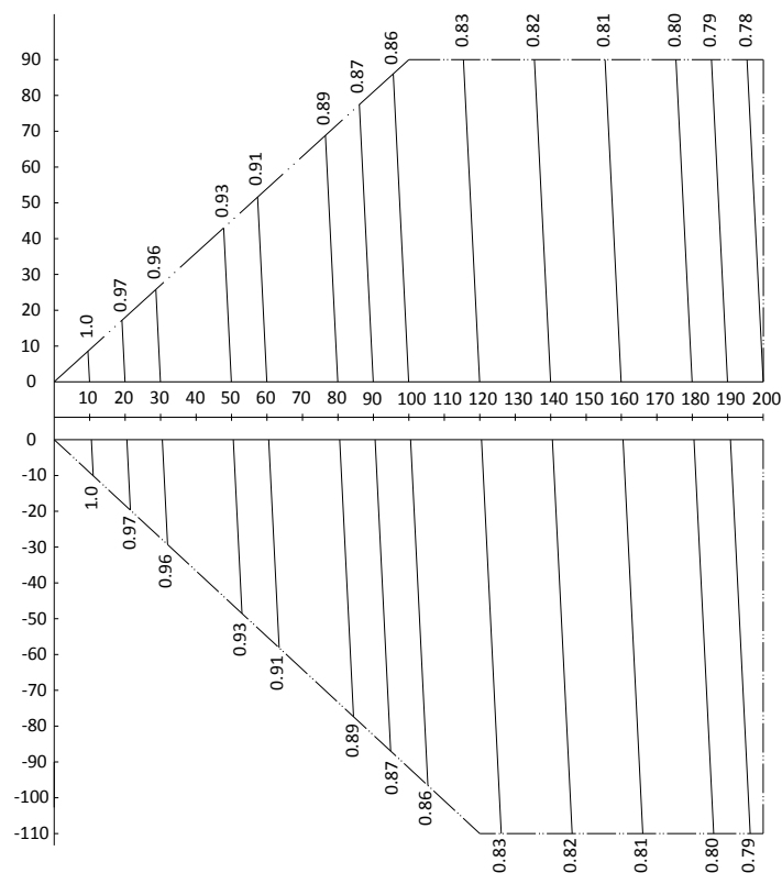
Figure 2-8.23: MVD-V5X1455(1510, 1565)W/V2GN1 rate of change in cooling capacity
