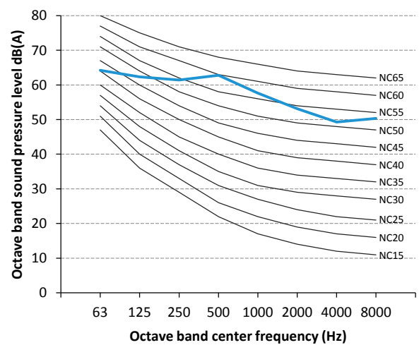
Figure 2-10.9 MVD-V5X615W/V2GN1 octave band level
