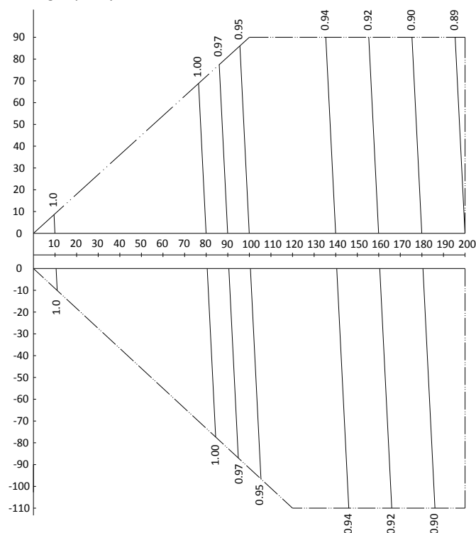
Figure 2-8.28: MVD-V5X1680(1730)W/V2GN1 rate of change in heating capacity
