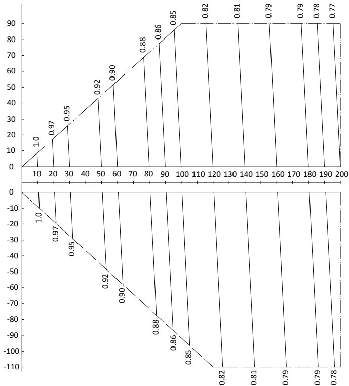
Figure 2-8.37: MVD-V5X2230W/V2GN1 rate of change in cooling capacity
