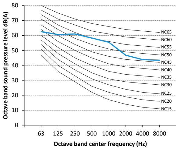
Figure 2-10.4 MVD-V5X335W/V2GN1 octave band level
