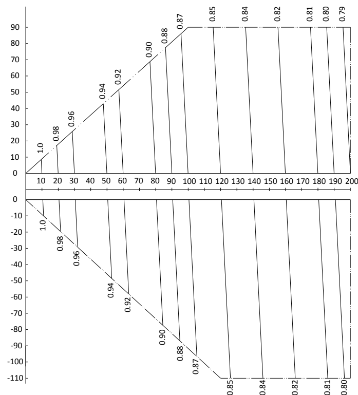
Figure 2-8.31: MVD-V5X1900W/V2GN1 rate of change in cooling capacity
