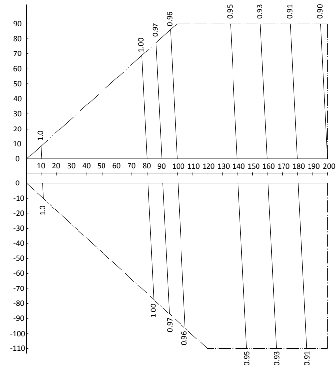
Figure 2-8.20: MVD-V5X1285W/V2GN1 rate of change in heating capacity
