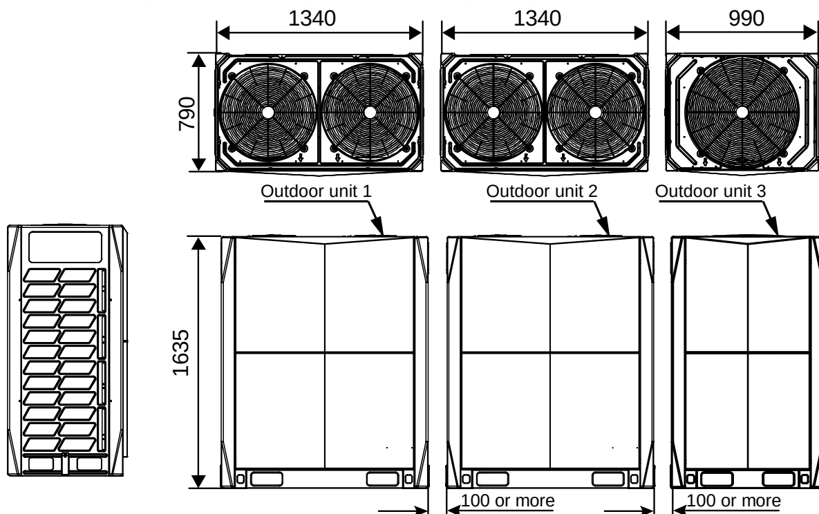
Figure 2-2.7: MVD-V5X1345(1395, 1455, 1510, 1565)W/V2GN1 dimensions (unit: mm)
