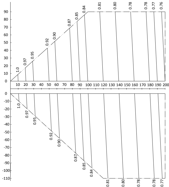
Figure 2-8.5: MVD-V5X560(615)W/V2GN1 rate of change in cooling capacity
