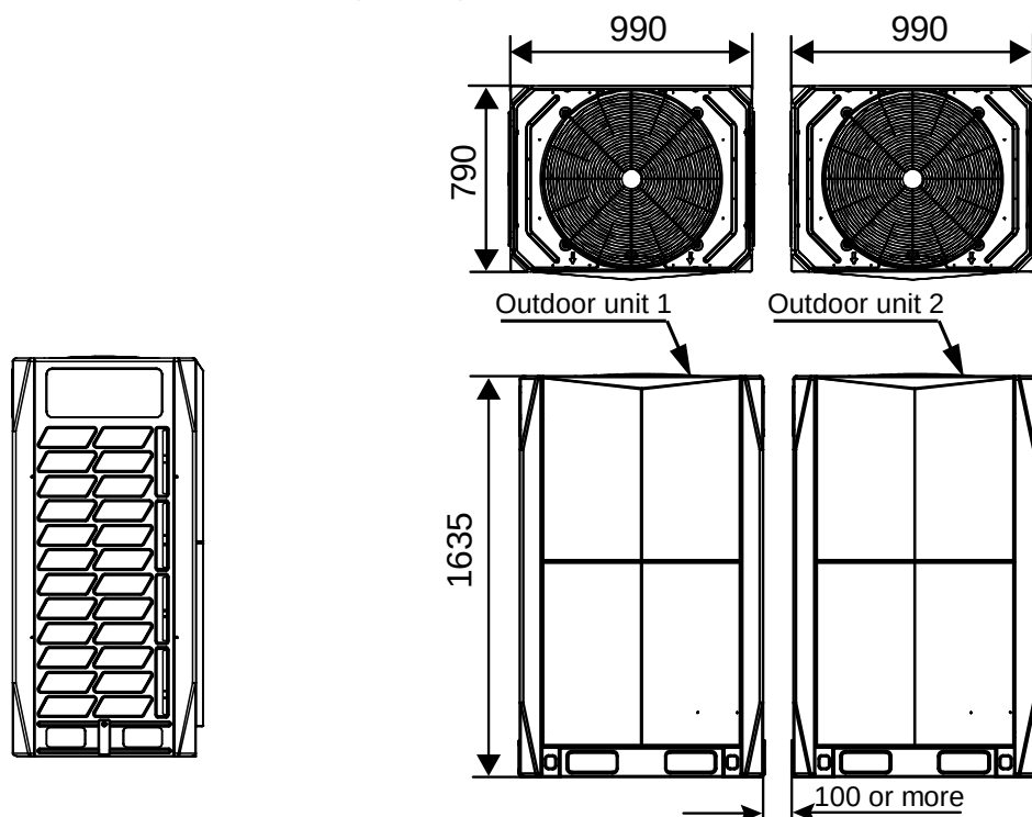
Figure 2-2.3: MVD-V5X670W/V2GN1 dimensions (unit: mm)
