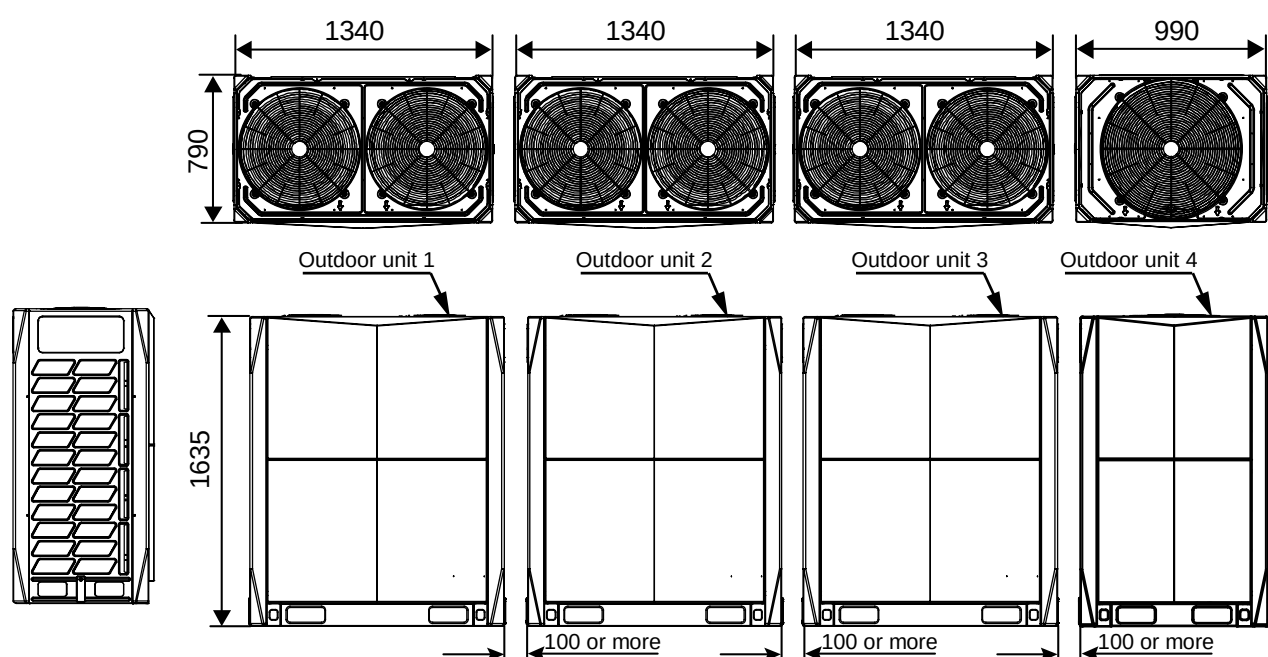
Figure 2-2.10 MVD-V5X1960(2010, 2070, 2125, 2180)W/V2GN1 dimensions (unit: mm)
