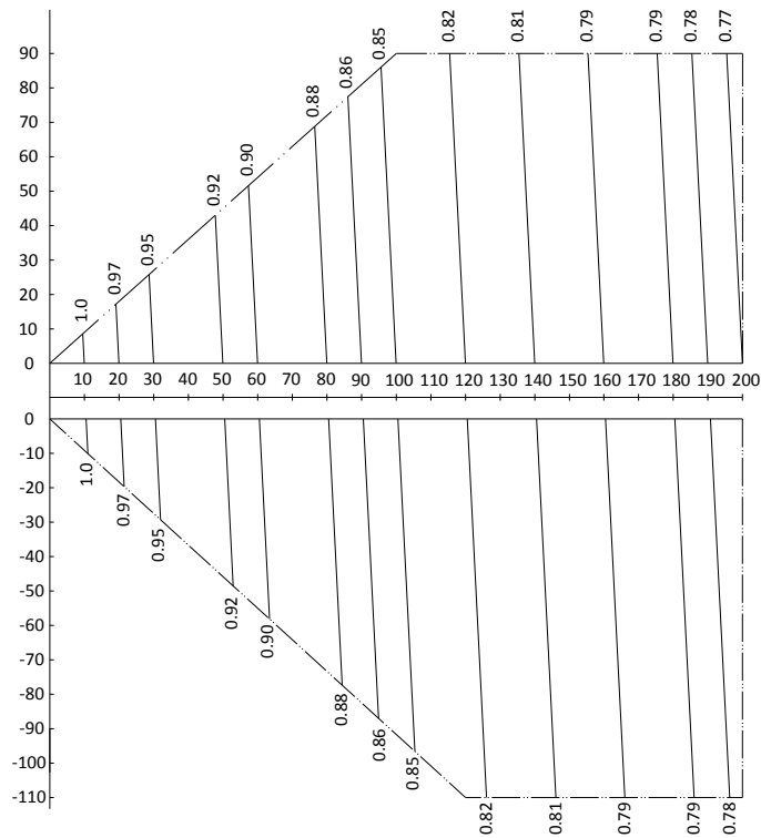
Figure 2-8.25: MVD-V5X1615W/V2GN1 rate of change in cooling capacity
