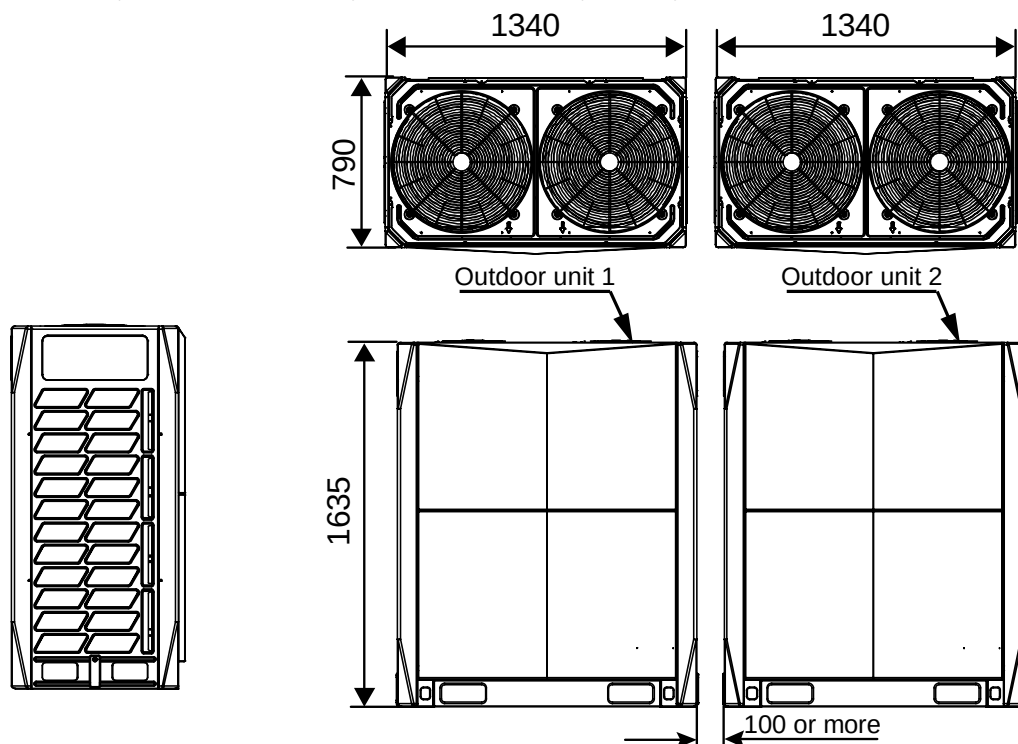
Figure 2-2.5: MVD-V5X1000(1065, 1115, 1175, 1230)W/V2GN1 dimensions (unit: mm)
