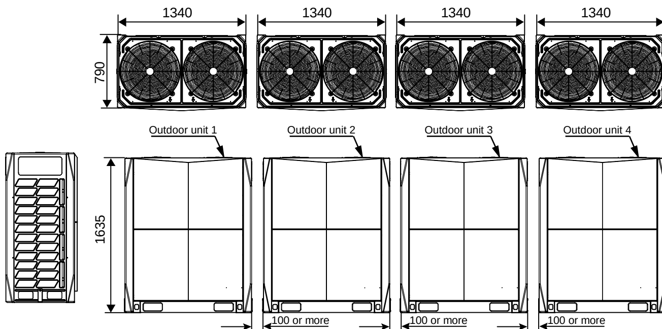
Figure 2-2.11 MVD-V5X2230(2295, 2345, 2405, 2460)W/V2GN1 dimensions (unit: mm)
