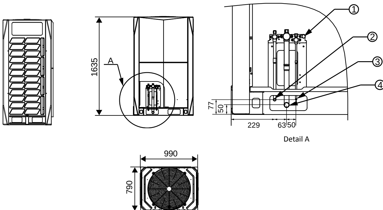
Figure 2-2.1: MVD-V5X252(280, 335)W/V2GN1 dimensions (unit: mm)
