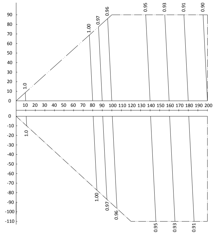
Figure 2-8.22: MVD-V5X1345(1395)W/V2GN1 rate of change in heating capacity
