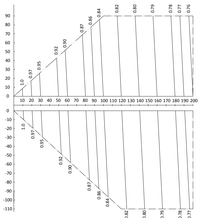
Figure 2-8.27: MVD-V5X1680(1730)W/V2GN1 rate of change in cooling capacity
