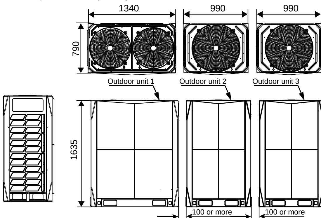
Figure 2-2.6: MVD-V5X1285W/V2GN1 dimensions (unit: mm)
