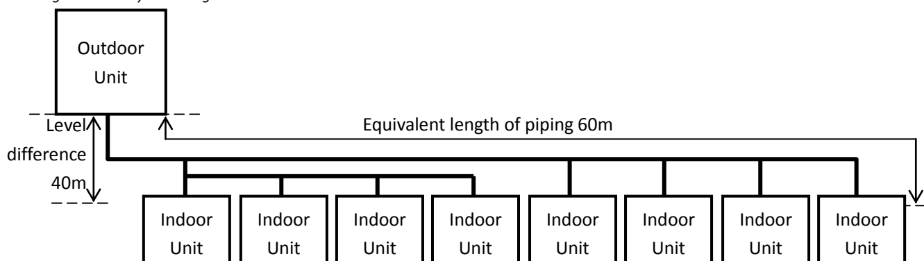
Figure 1-6.2: System diagram
