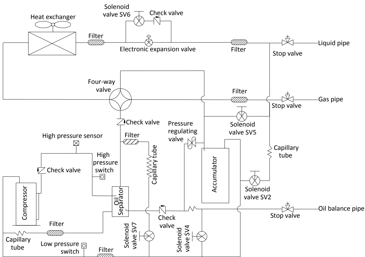
Figure 2-4.1: MVD-V5X252(280, 335)W/V2GN1 piping diagram
