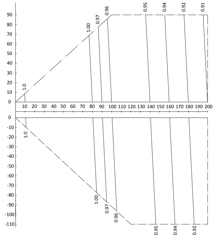
Figure 2-8.10: MVD-V5X730(780)W/V2GN1 rate of change in heating capacity
