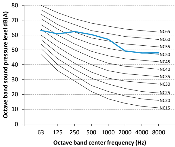
Figure 2-10.6 MVD-V5X450W/V2GN1 octave band level
