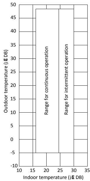
Figure 2-9.1: Cooling operating limit
