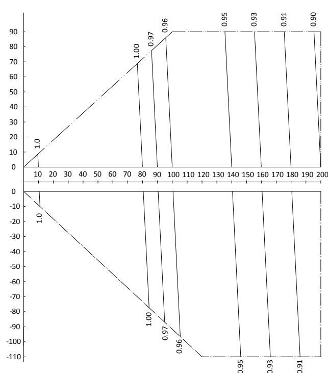
Figure 2-8.16: MVD-V5X1065(1115)W/V2GN1 rate of change in heating capacity
