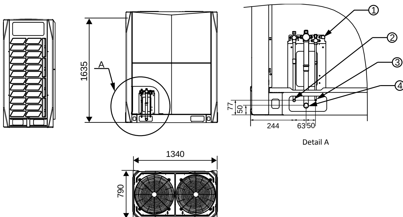
Figure 2-2.2: MVD-V5X400(450, 500, 560, 615)W/V2GN1 dimensions (unit: mm)
