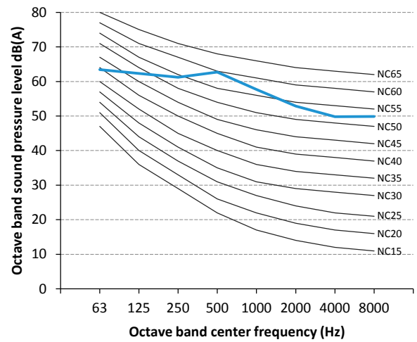
Figure 2-10.7 MVD-V5X500W/V2GN1 octave band level
