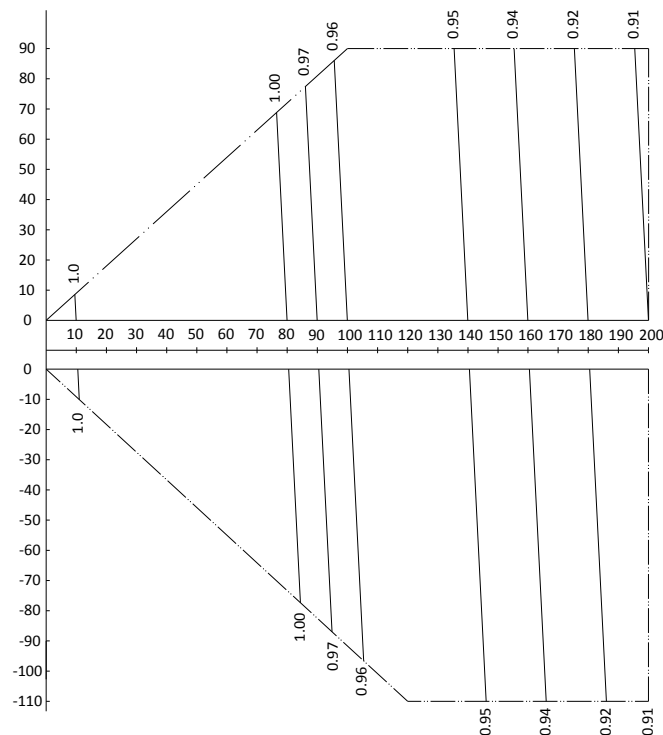
Figure 2-8.8: MVD-V5X670W/V2GN1 rate of change in heating capacity
