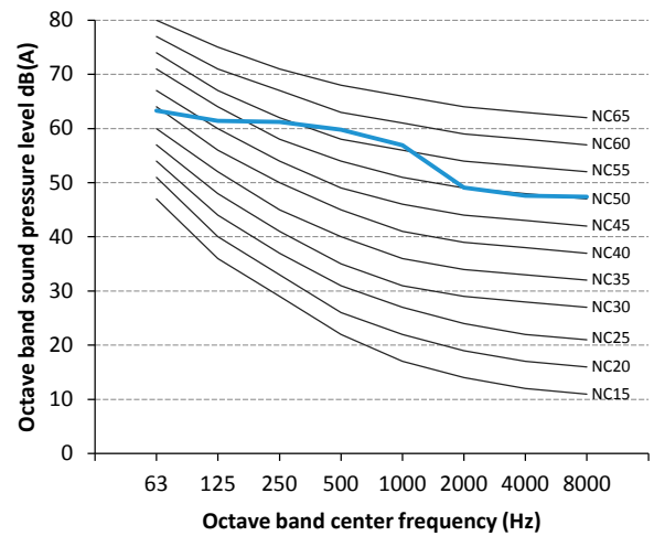
Figure 2-10.5 MVD-V5X400W/V2GN1 octave band level
