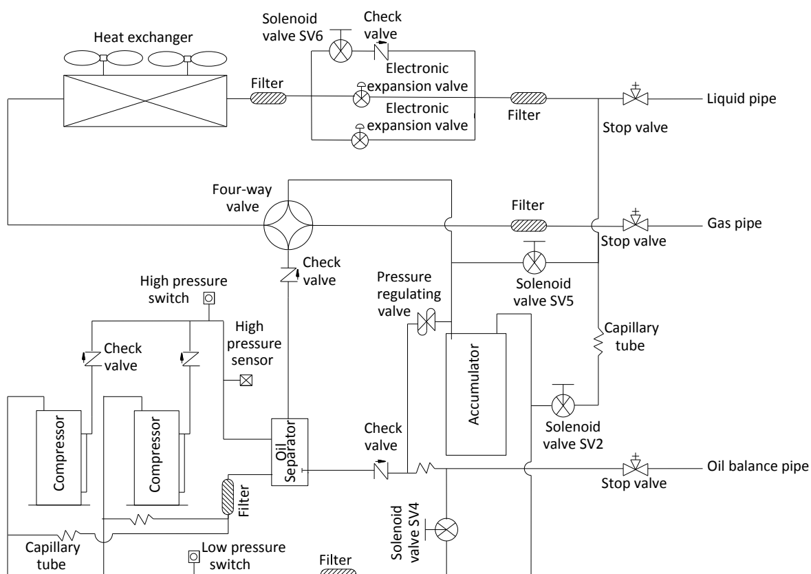
Figure 2-4.2: MVD-V5X400(450)W/V2GN1 piping diagram
