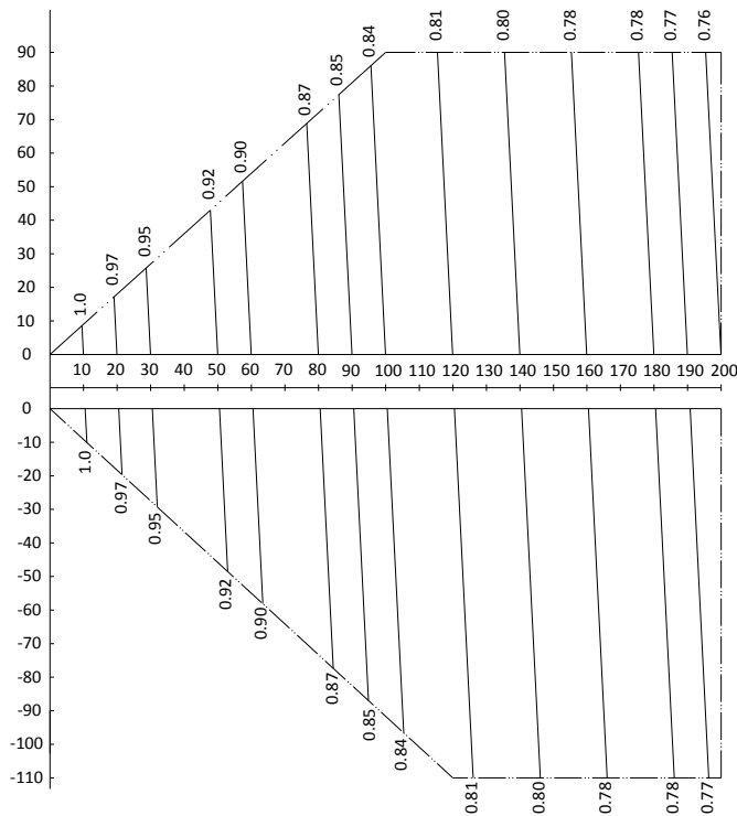
Figure 2-8.41: MVD-V5X2405(2460)W/V2GN1 rate of change in cooling capacity
