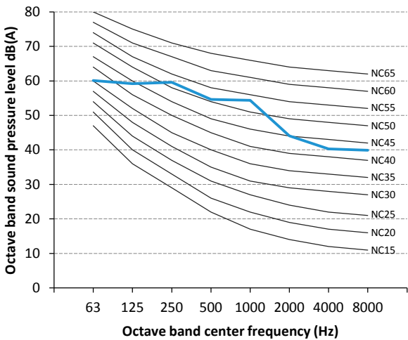
Figure 2-10.2 MVD-V5X252W/V2GN1 octave band level
