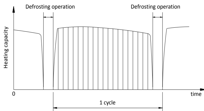
Figure 2-8.43: Defrosting cycle
