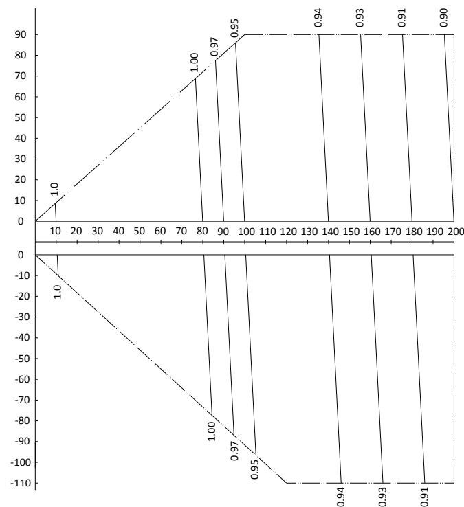
Figure 2-8.24: MVD-V5X1455(1510, 1565)W/V2GN1 rate of change in heating capacity
