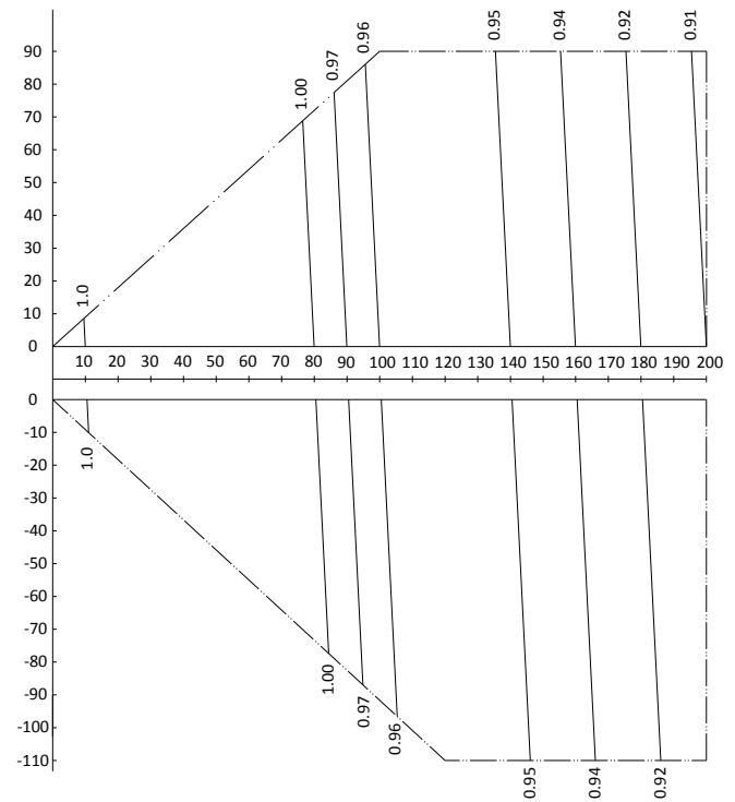
Figure 2-8.2: MVD-V5X252(280, 335)W/V2GN1 rate of change in heating capacity
