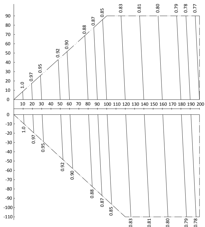
Figure 2-8.3: MVD-V5X400(450, 500)W/V2GN1 rate of change in cooling capacity
