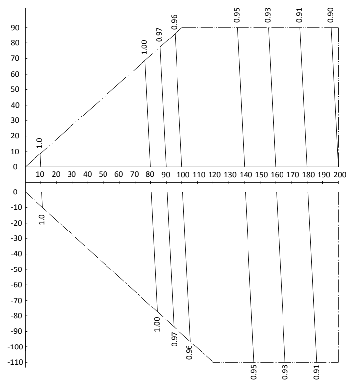
Figure 2-8.14: MVD-V5X1000W/V2GN1 rate of change in heating capacity
