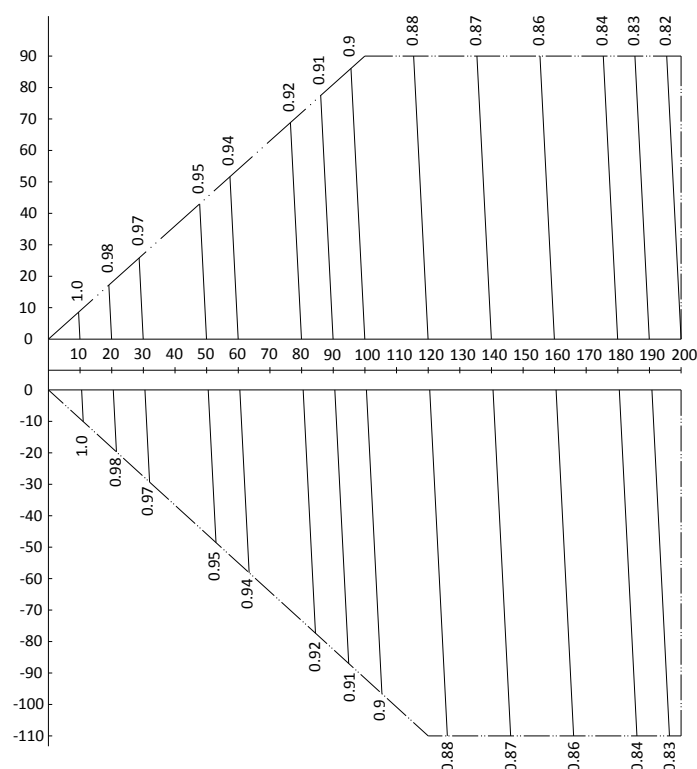
Figure 2-8.7: MVD-V5X670W/V2GN1 rate of change in cooling capacity
