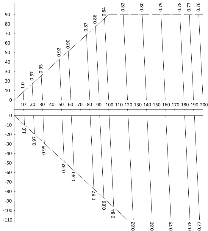
Figure 2-8.39: MVD-V5X2295(2345)W/V2GN1 rate of change in cooling capacity
