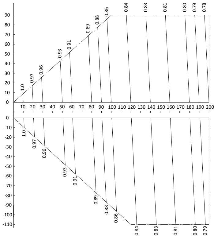
Figure 2-8.21: MVD-V5X1345(1395)W/V2GN1 rate of change in cooling capacity
