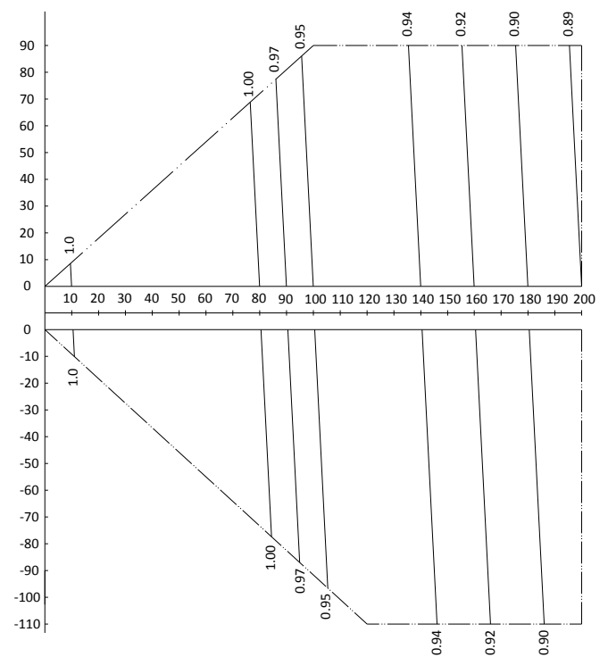
Figure 2-8.40: MVD-V5X2295(2345)W/V2GN1 rate of change in heating capacity
