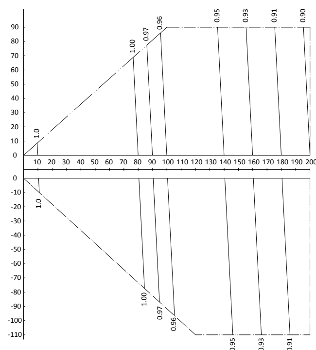
Figure 2-8.12: MVD-V5X840(895, 950)W/V2GN1 rate of change in heating capacity
