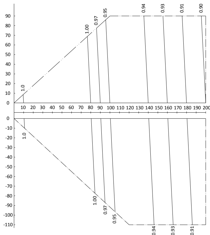
Figure 2-8.36: MVD-V5X2070(2125, 2180)W/V2GN1 rate of change in heating capacity
