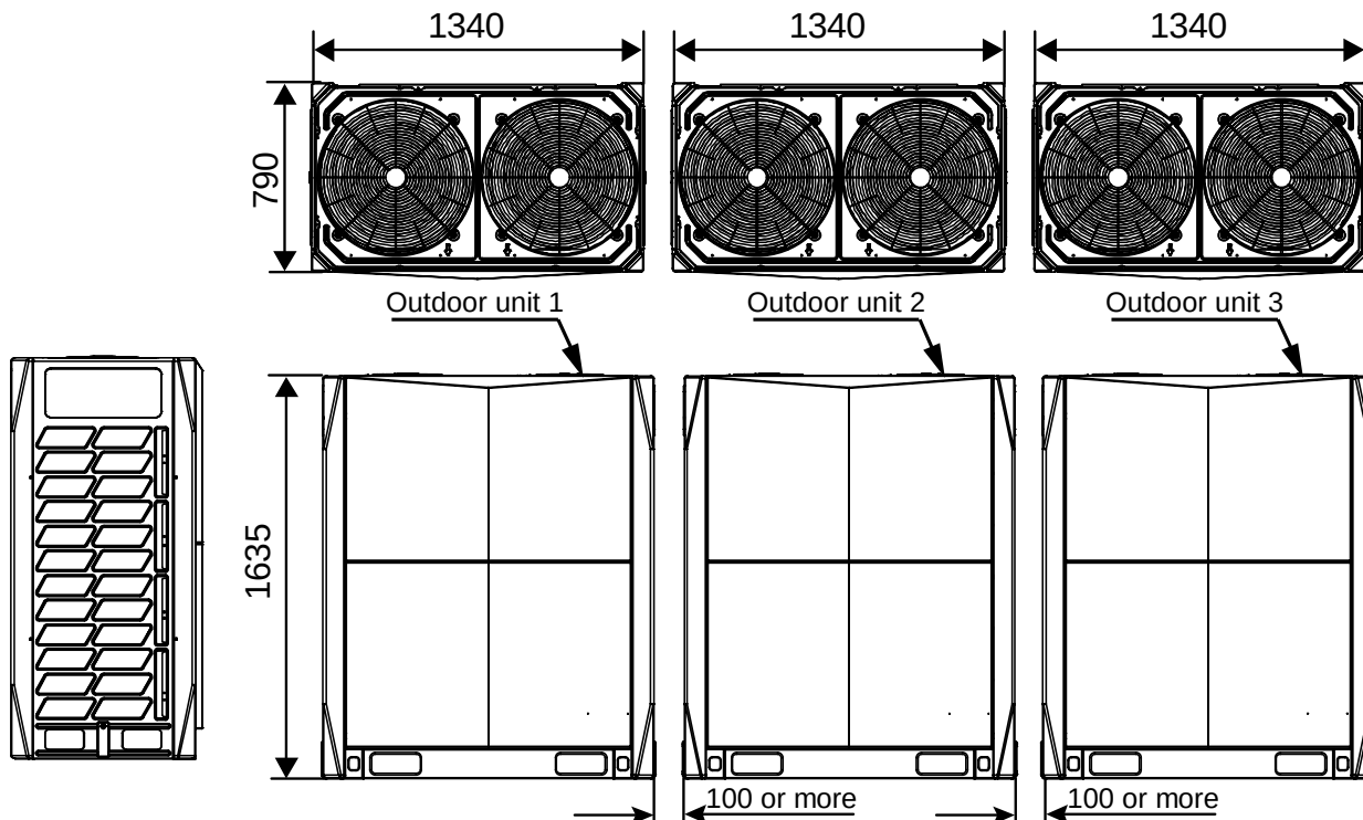
Figure 2-2.8: MVD-V5X1615(1680, 1730, 1790, 1845)W/V2GN1 dimensions (unit: mm)
