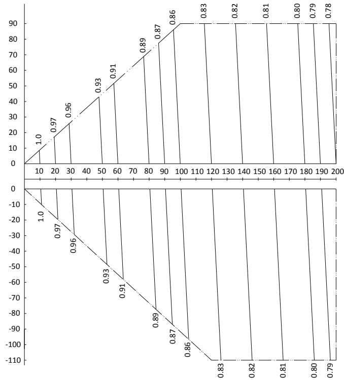
Figure 2-8.33: MVD-V5X1960(2010)W/V2GN1 rate of change in cooling capacity
