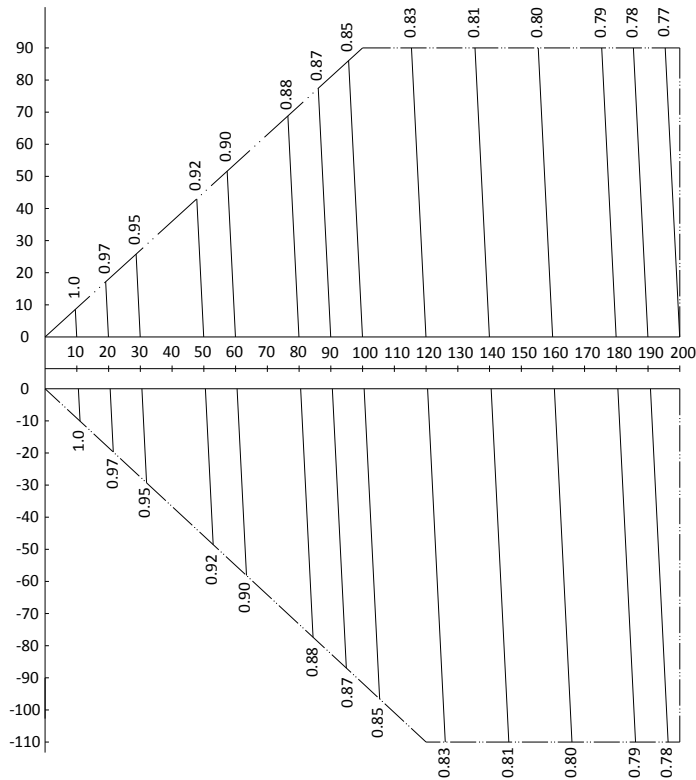
Figure 2-8.13: MVD-V5X1000W/V2GN1 rate of change in cooling capacity
