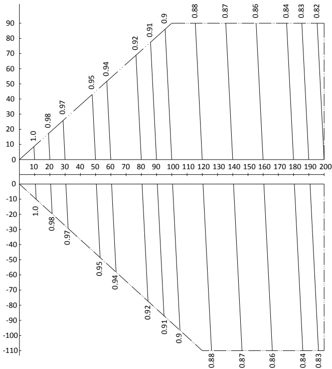
Figure 2-8.1: MVD-V5X252(280, 335)W/V2GN1 rate of change in cooling capacity
