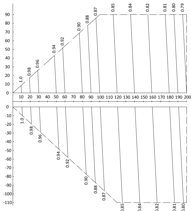
Figure 2-8.11: MVD-V5X840(895, 950)W/V2GN1 rate of change in cooling capacity
