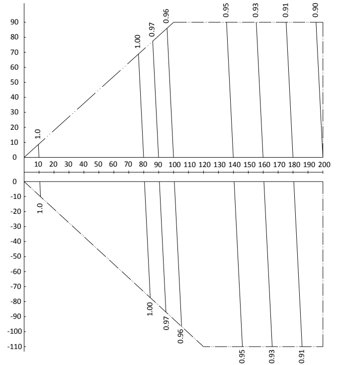
Figure 2-8.38: MVD-V5X2230W/V2GN1 rate of change in heating capacity
