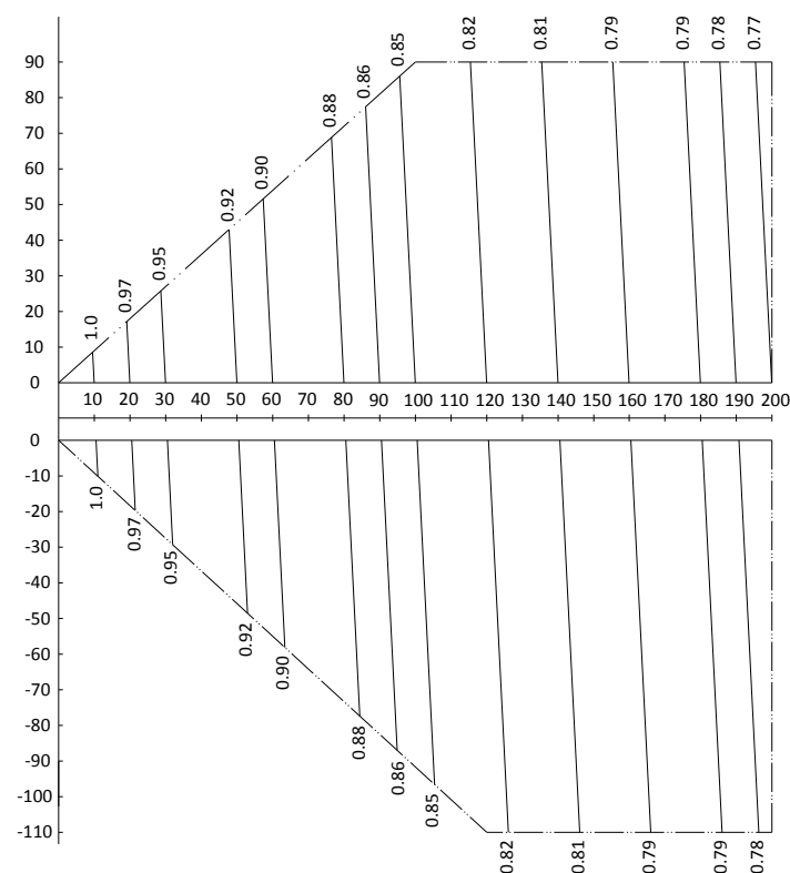
Figure 2-8.15: MVD-V5X1065(1115)W/V2GN1 rate of change in cooling capacity
