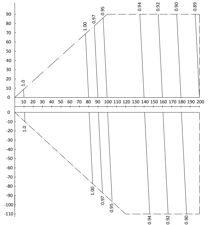
Figure 2-8.30: MVD-V5X1790(1845)W/V2GN1 rate of change in heating capacity
