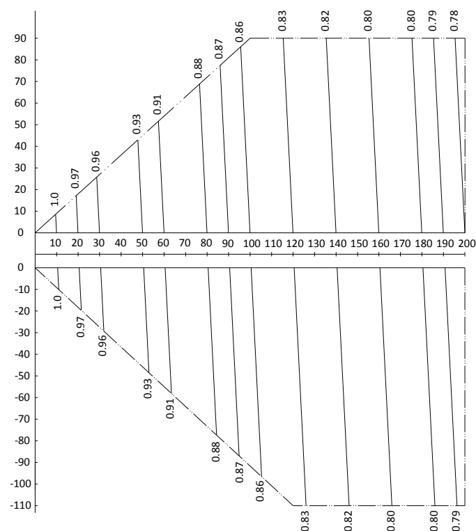
Figure 2-8.35: MVD-V5X2070(2125, 2180)W/V2GN1 rate of change in cooling capacity
