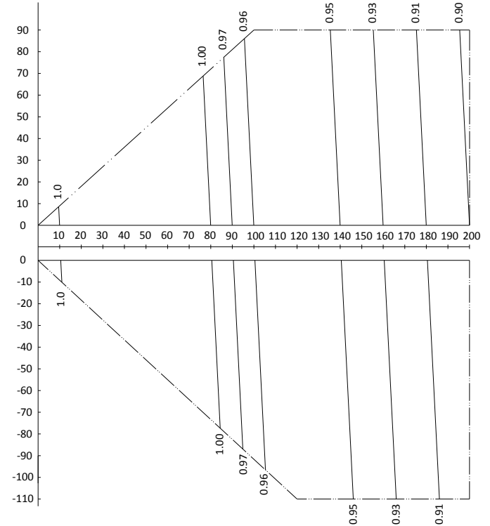
Figure 2-8.34: MVD-V5X1960(2010)W/V2GN1 rate of change in heating capacity
