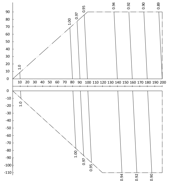
Figure 2-8.42: MVD-V5X2405(2460)W/V2GN1 rate of change in heating capacity
