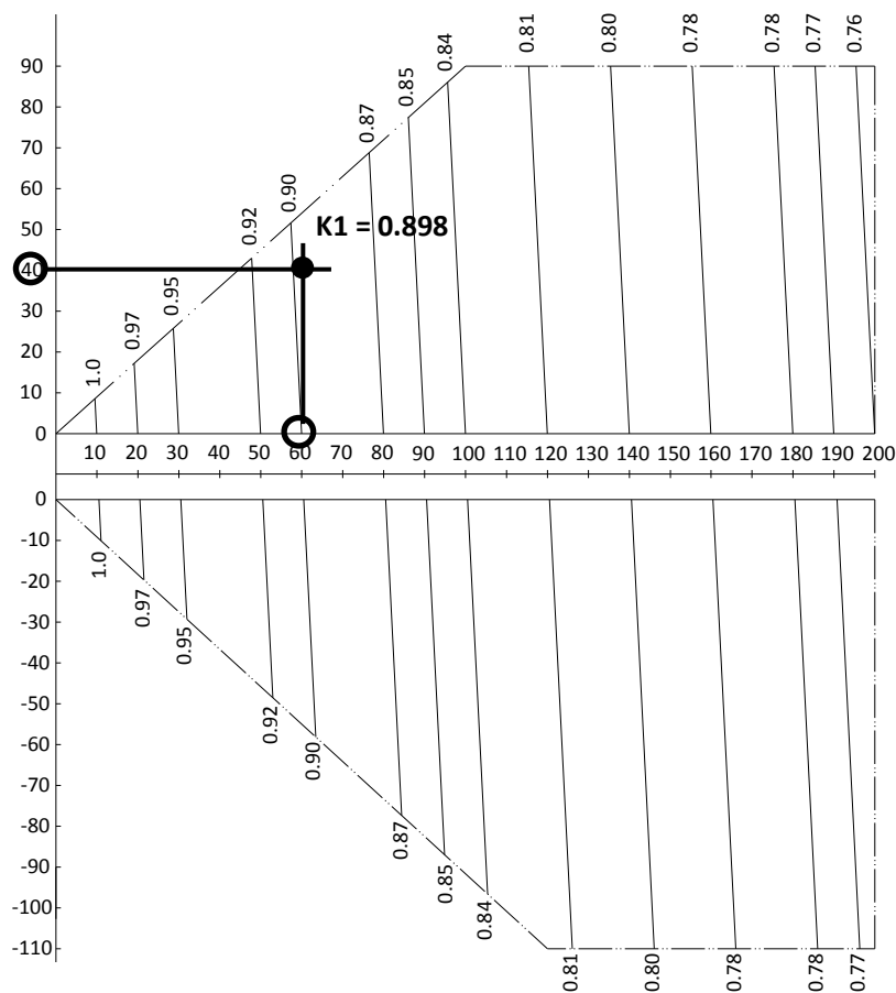
Figure 1-6.3: MV5-X560W/V2GN1 rate of change in cooling capacity
