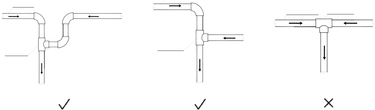
Figure 3-6.2: Drain piping joints – correct and incorrect configurations
