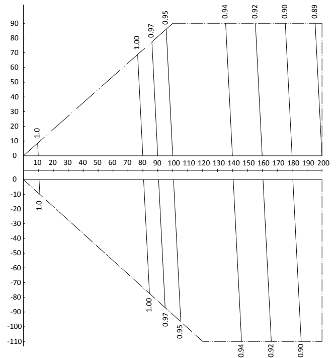
Figure 2-8.6: MVD-V5X560(615)W/V2GN1 rate of change in heating capacity
