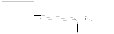
Figure 3-6.1: Drain piping minimum slope requirement
