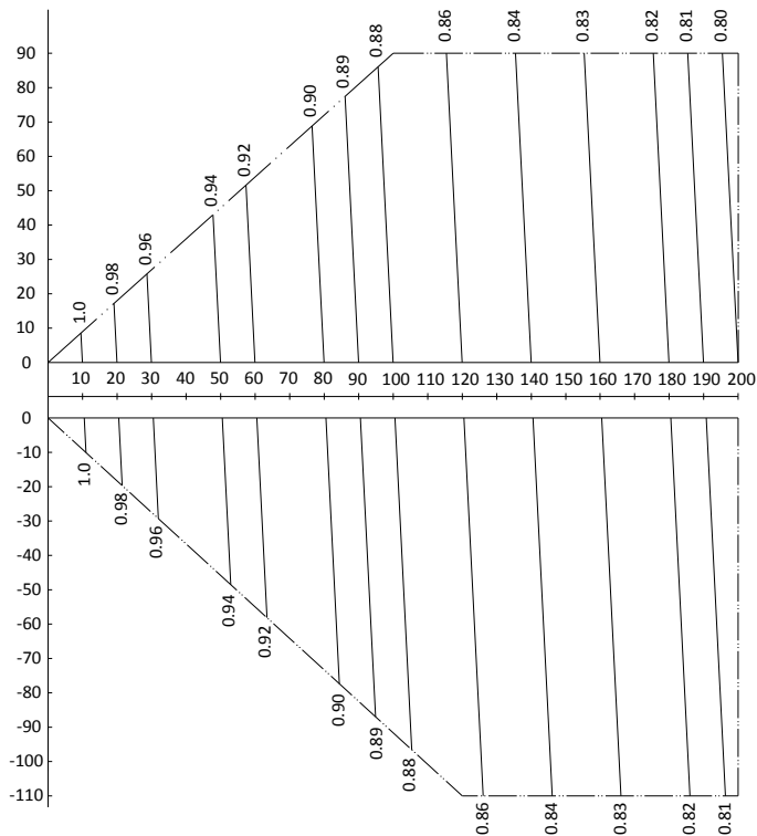
Figure 2-8.9: MVD-V5X730(780)W/V2GN1 rate of change in cooling capacity
