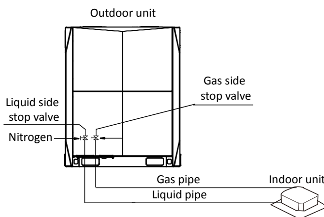
Figure 3-5.13: Gastightness test
