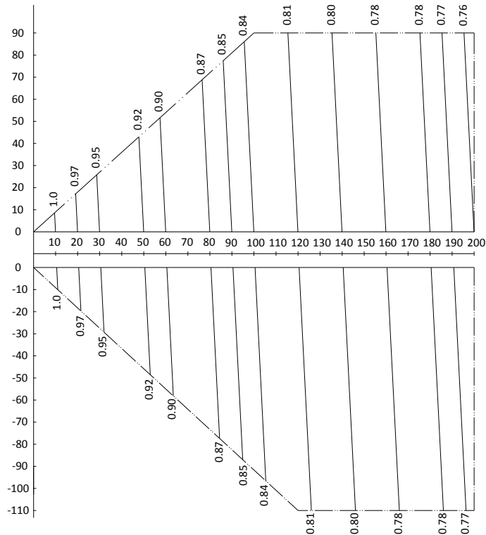
Figure 2-8.17: MVD-V5X1175(1230)W/V2GN1 rate of change in cooling capacity
