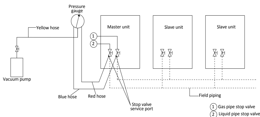
Figure 3-5.14: Vacuum drying
