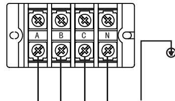
To 380-415V 3N- 50Hz/60Hz Fig.6-1
