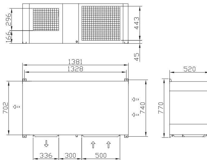
Dimensiones mods. 30 / 36
